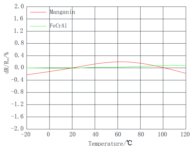
FIG.2: T.C.R Derating Curve
